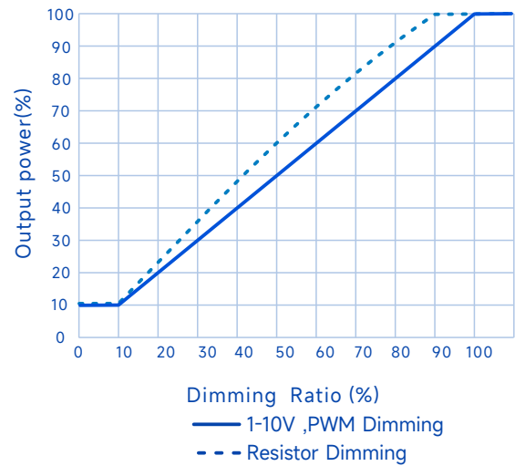
Output Power Vs. Dimming (BB models)
